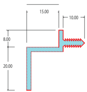
7501 ALUMINIUM INTERNAL FIXING PROFILE (To accommodate 53mm wall thickness)
