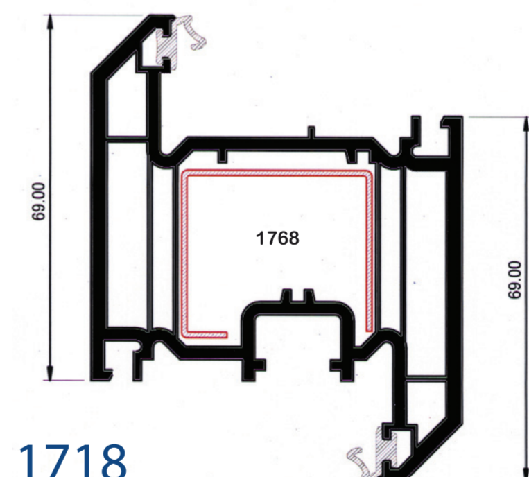
1714 Tilt and Turn Sash
