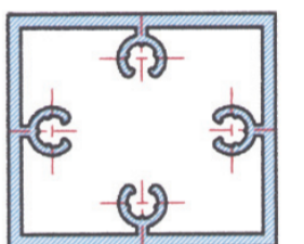
1761 Aluminium Reinforcement for 1712 Transom
