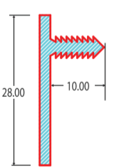
7500 ALUMINIUM INTERNAL FIXING PROFILE (To accommodate 38mm wall thickness)
